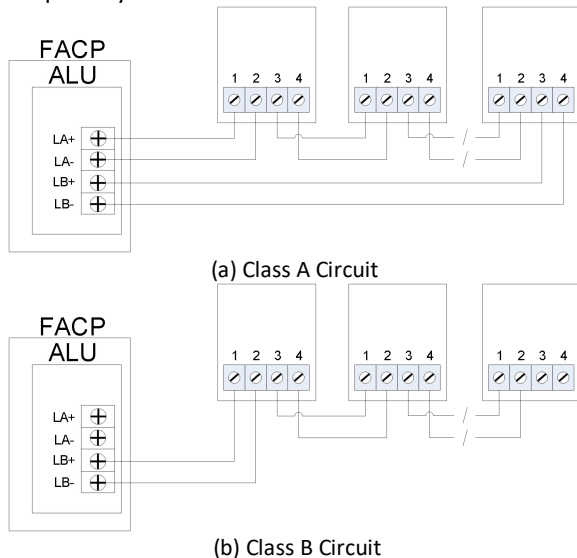
(b) Class B Circuit Figure 2. Wiring Diagram
