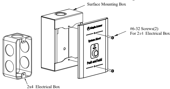
Figure 1. Abort Switch Installation
